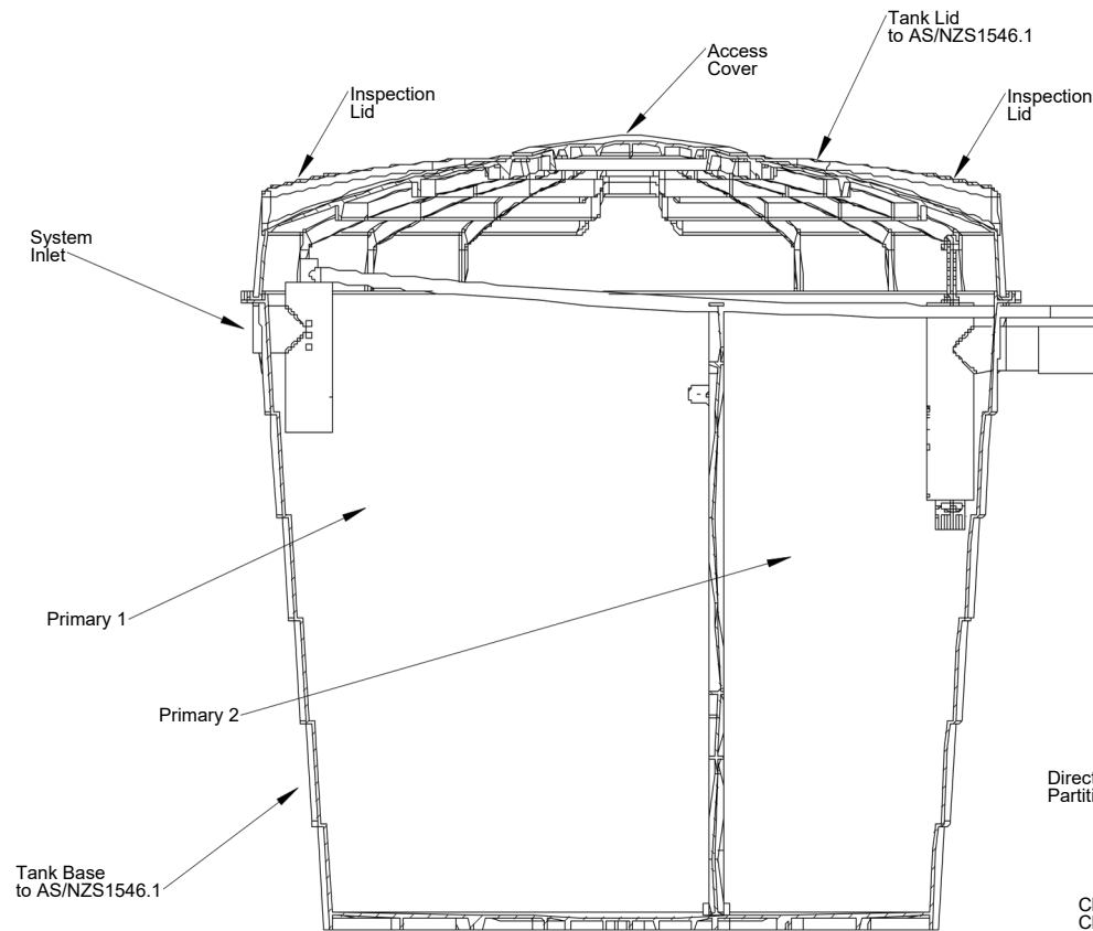
Primary Treatment Tank
