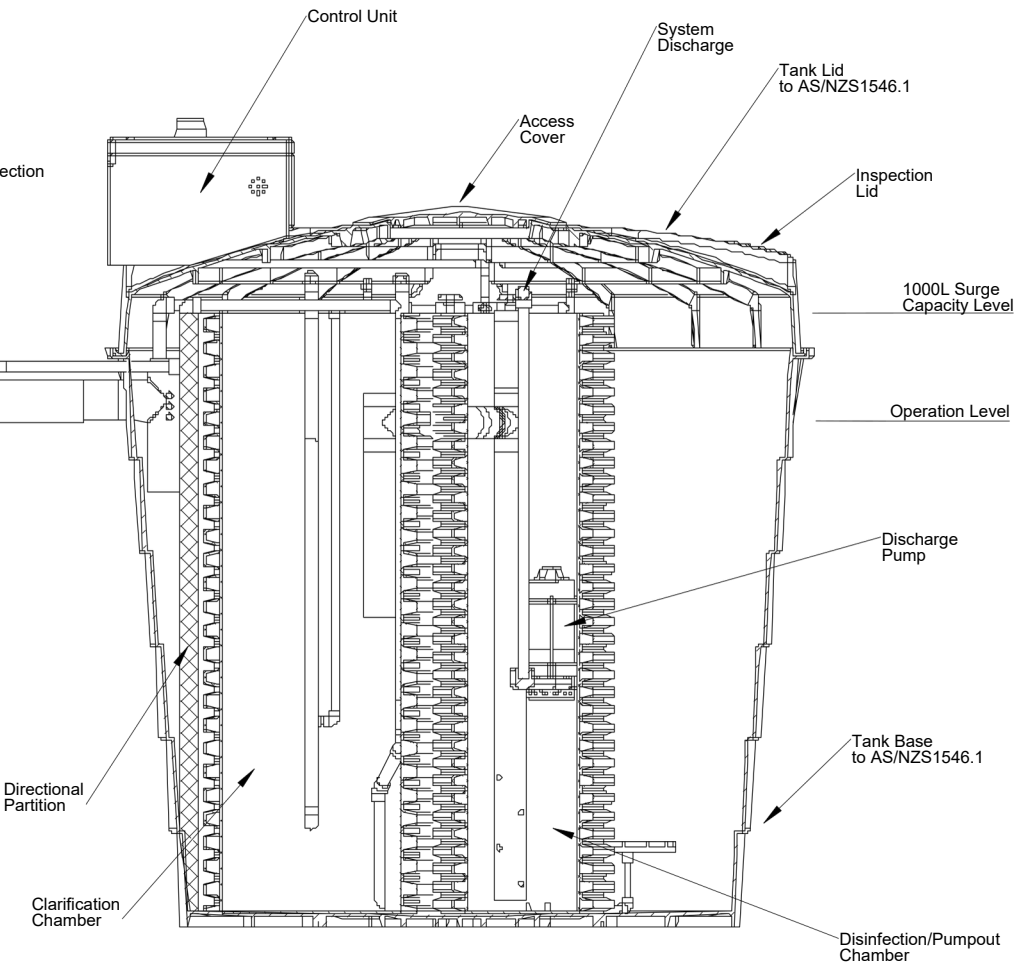
Advanced Secondary Treatment Tank
